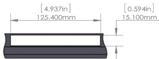
Commercial Operator Cutout
