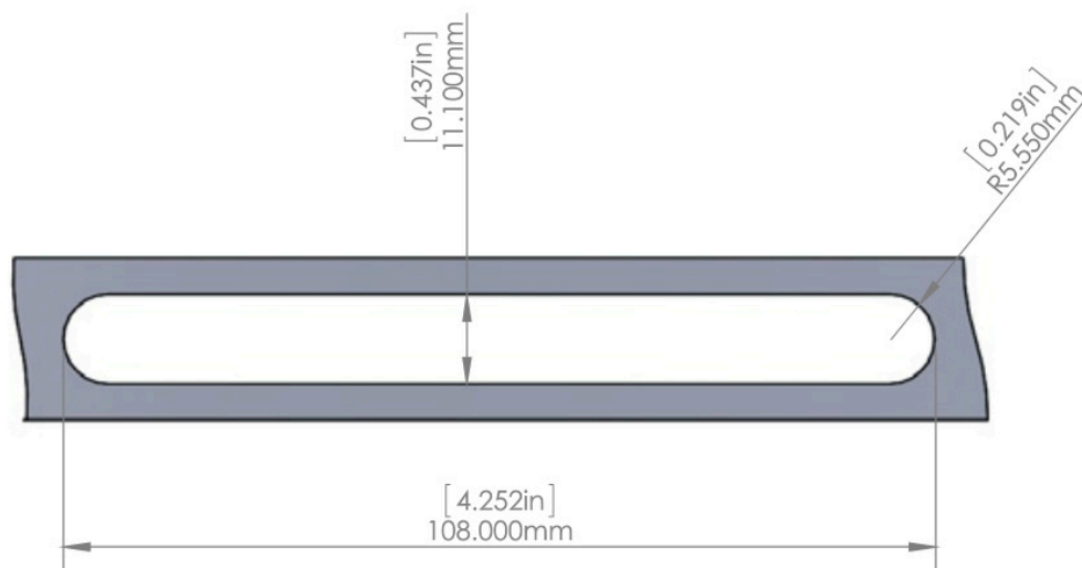
Locking Handle Cutout
