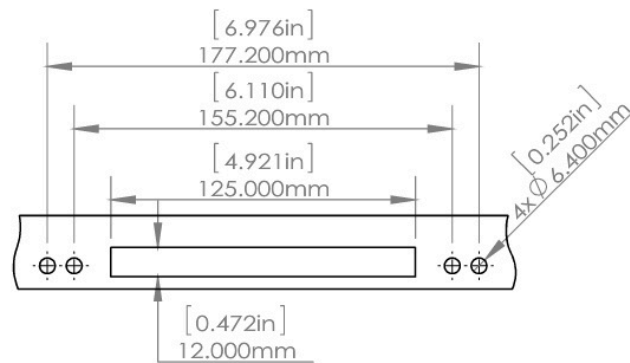
Residential Operator Cutout
